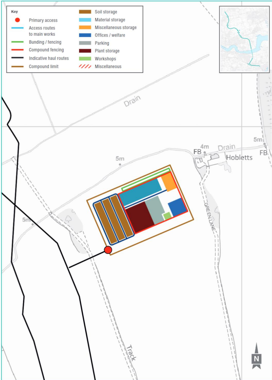
Plate 1.13 Indicative layout for Mardyke compound
