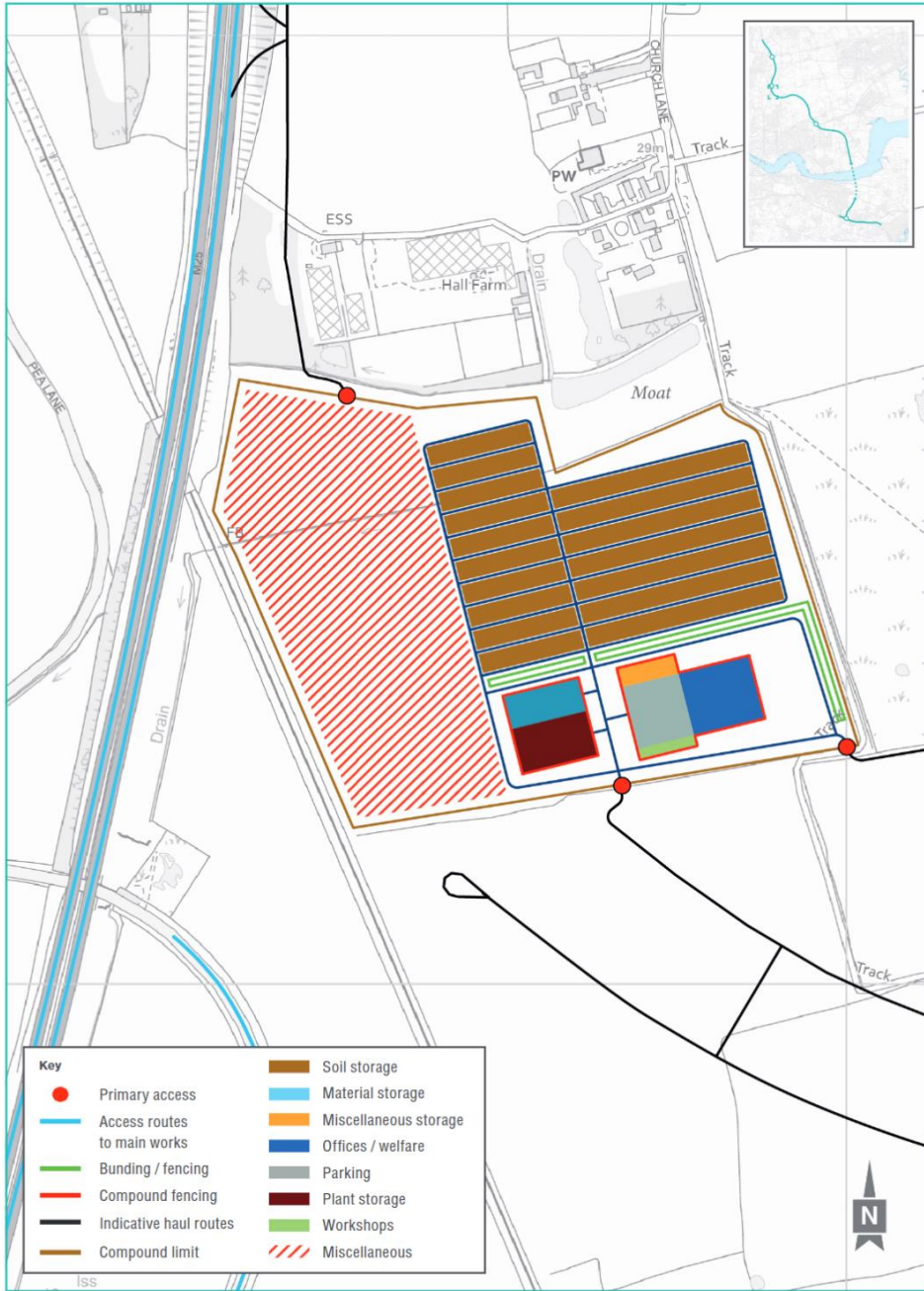
Plate 1.15 Indicative layout for M25 compound
