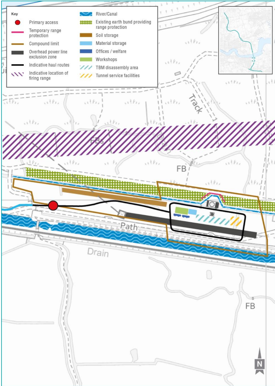
Plate 1.5 Indicative layout for Milton compound
