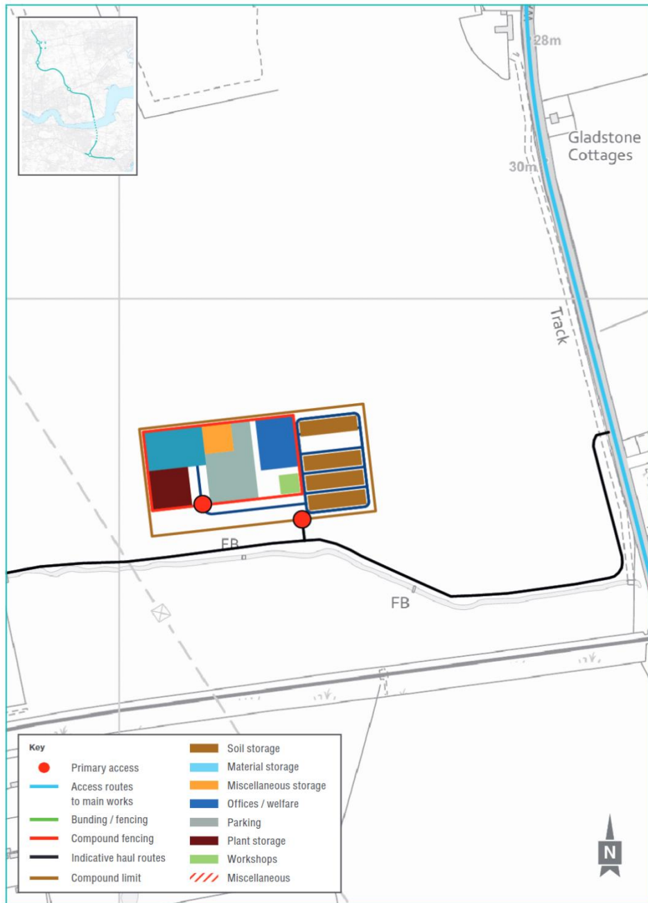
Plate 1.17 Indicative layout for Warley Street compound
