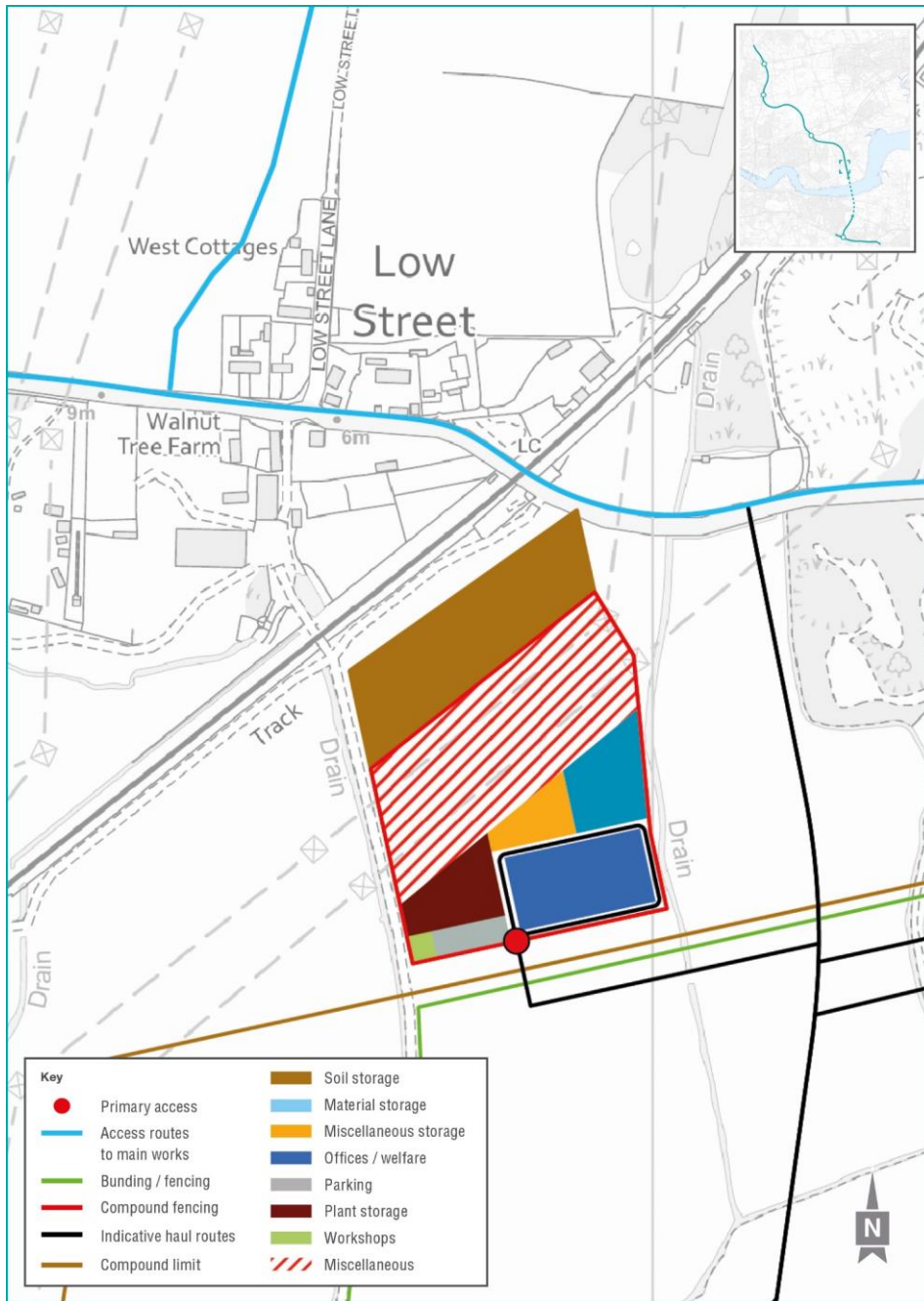
Plate 1.7 Indicative layout for Station Road compound
