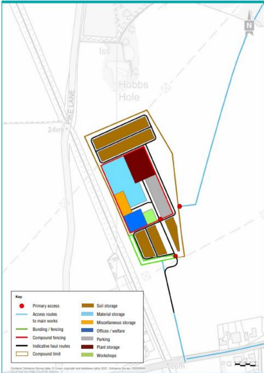
Plate 1.16 Indicative layout for Ockendon Road compound
