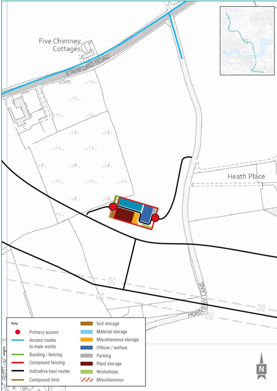
Plate 1.9 Indicative layout for Stanford Road compound
