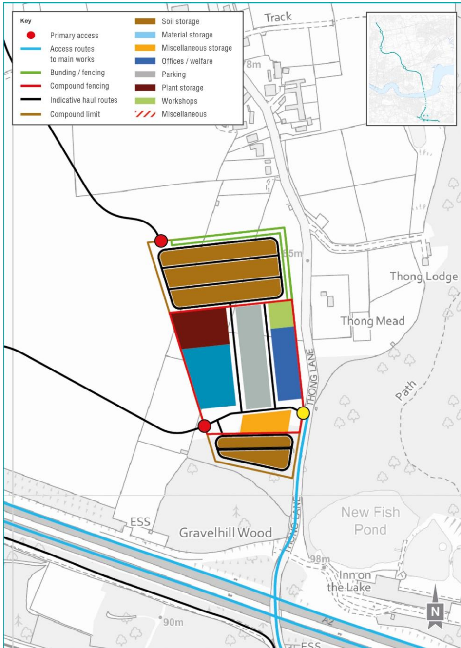
Plate 1.2 Indicative layout for A2 compound
