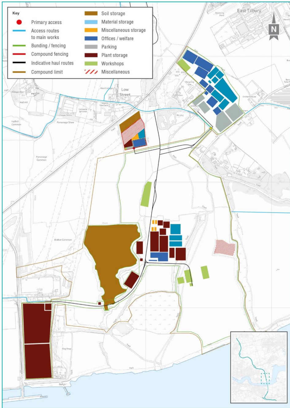
Plate 1.6 Indicative layout for Northern tunnel entrance compound
