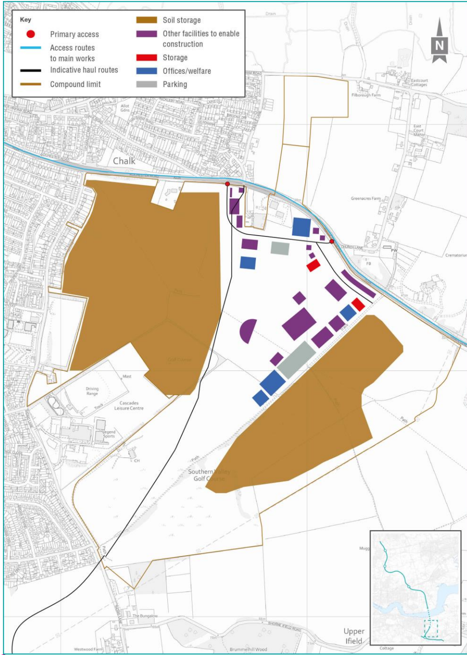
Plate 1.3 Indicative layout for Southern tunnel entrance compound
