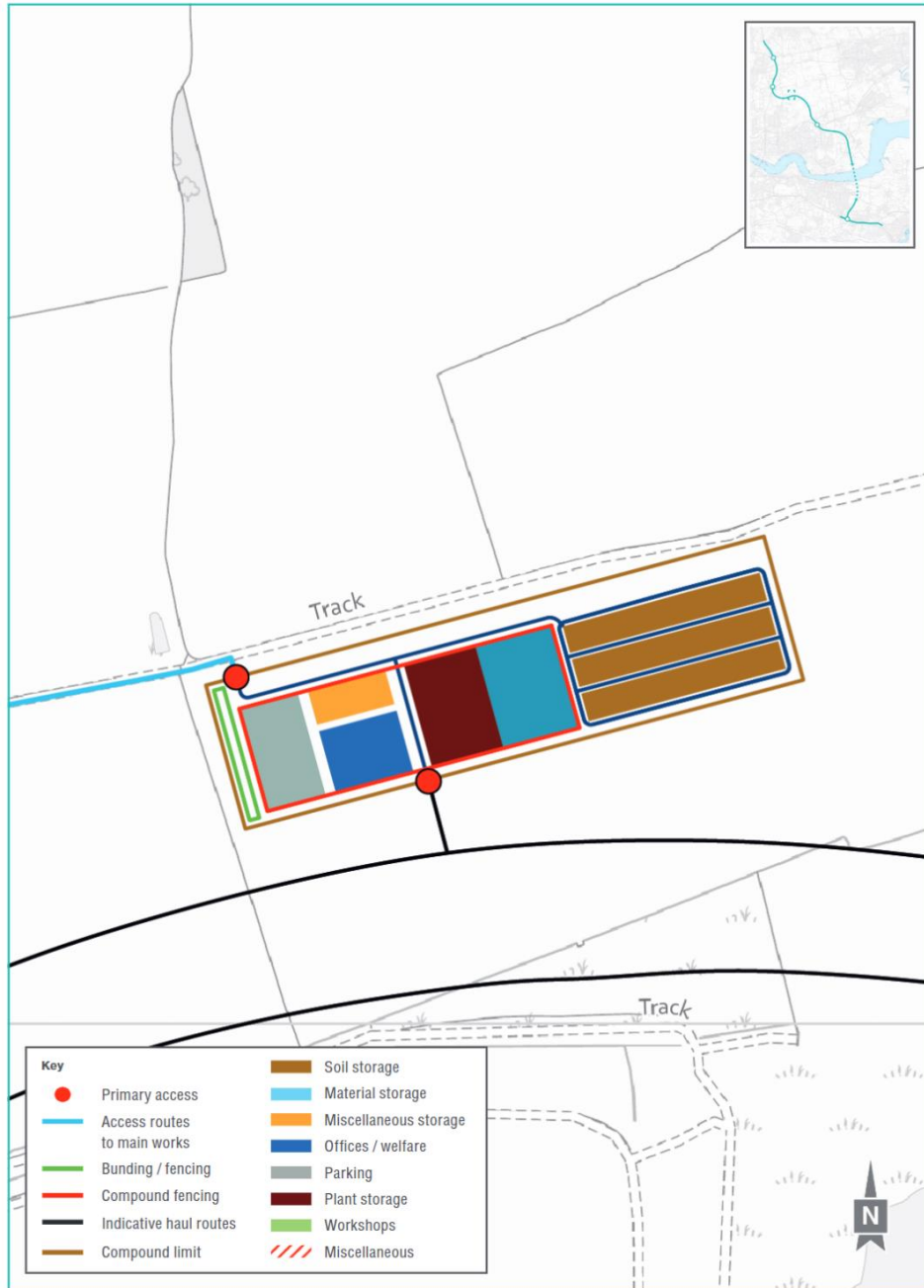
Plate 1.14 Indicative layout for Medebridge compound
