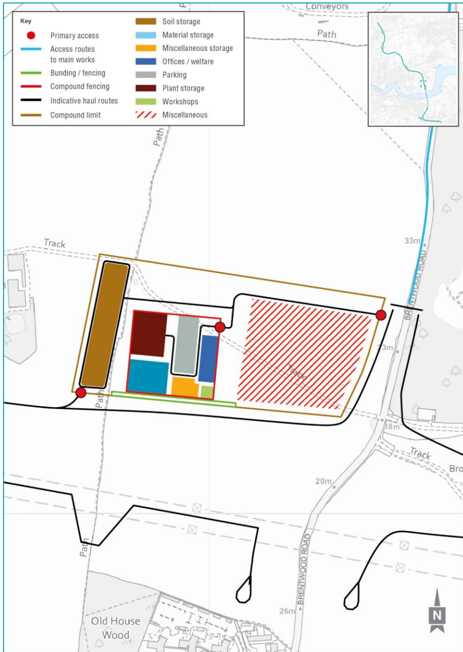
Plate 1.8 Indicative layout for Brentwood Road compound
