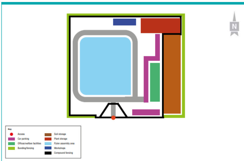
Plate 1.19 Utility Logistics Hub alternative indicative layout
