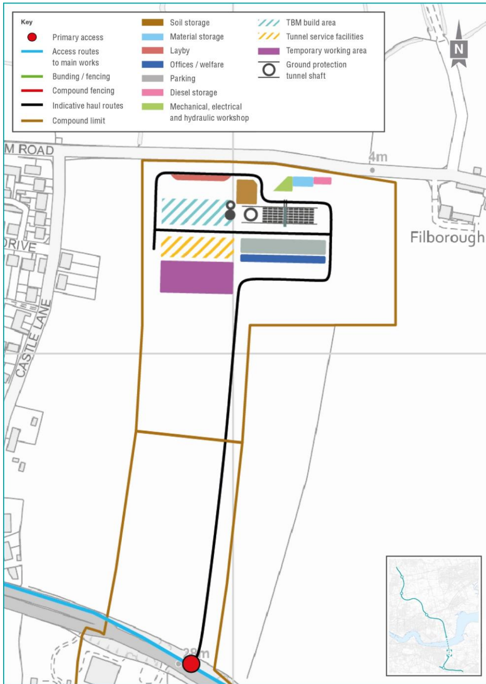
Plate 1.4 Indicative layout for A226 Gravesend Road compound
